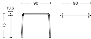
PALISSADE MIDDLE LEG Width 90 cm Depth 13,5 cm Height 75 cm Weight 3,48 kg
